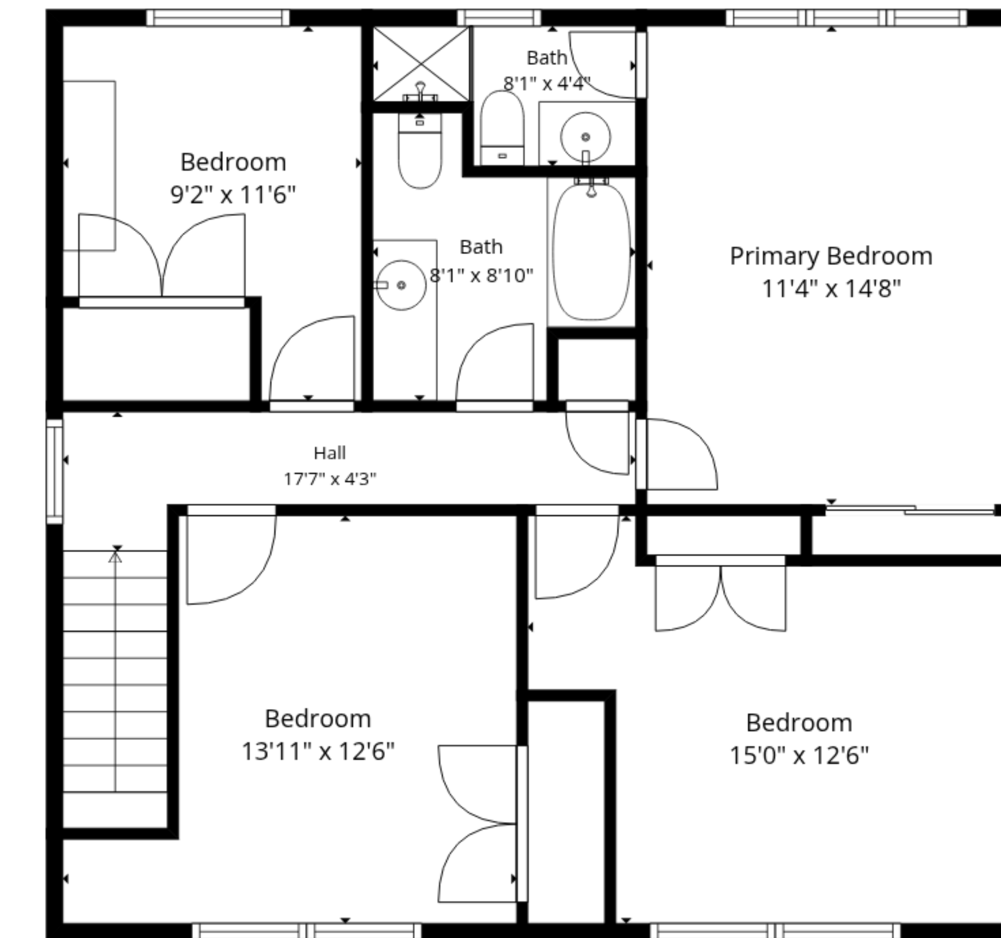
2nd Floor
