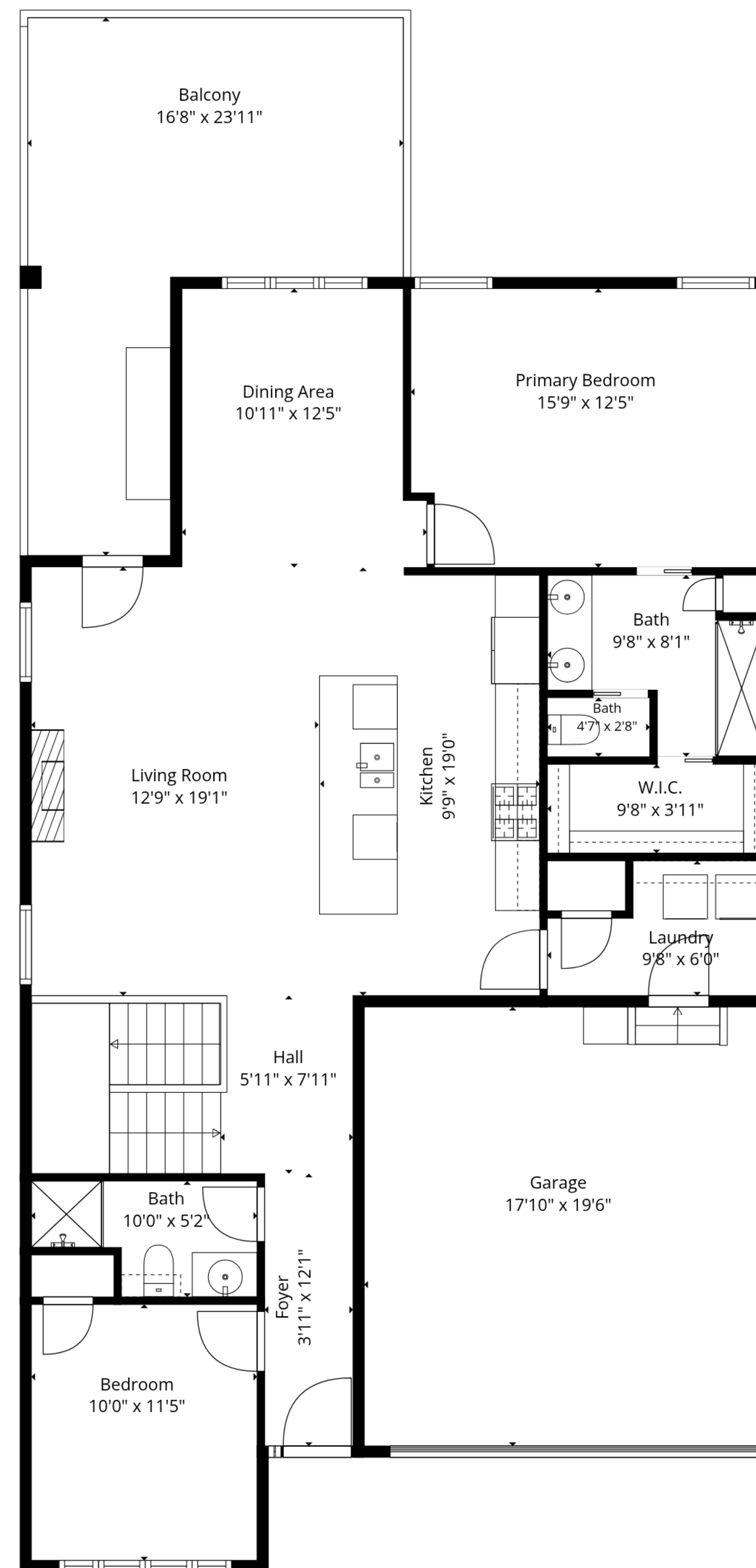
1st Floor
