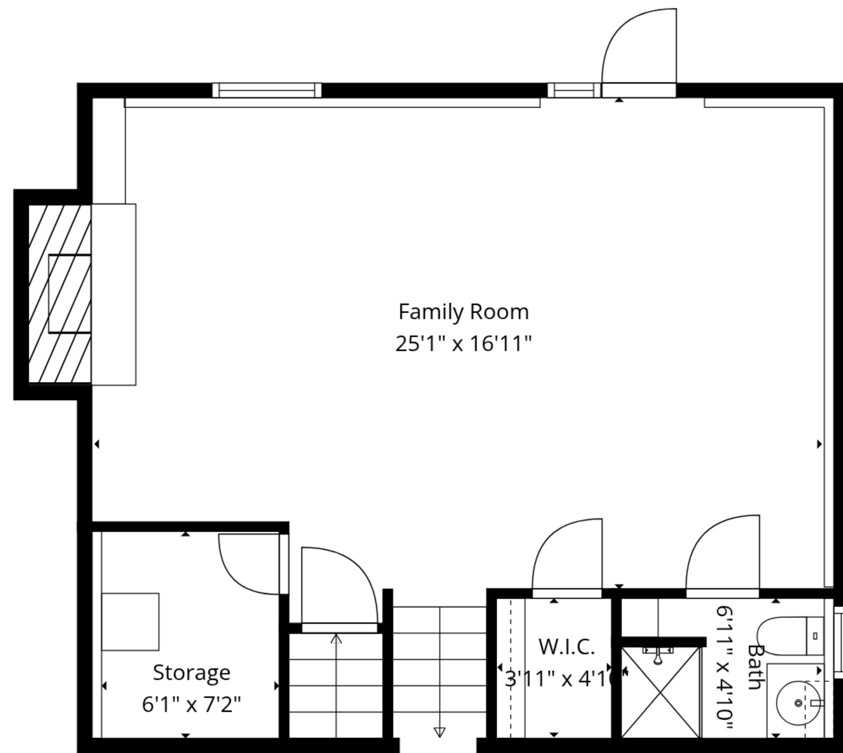
1st Floor
