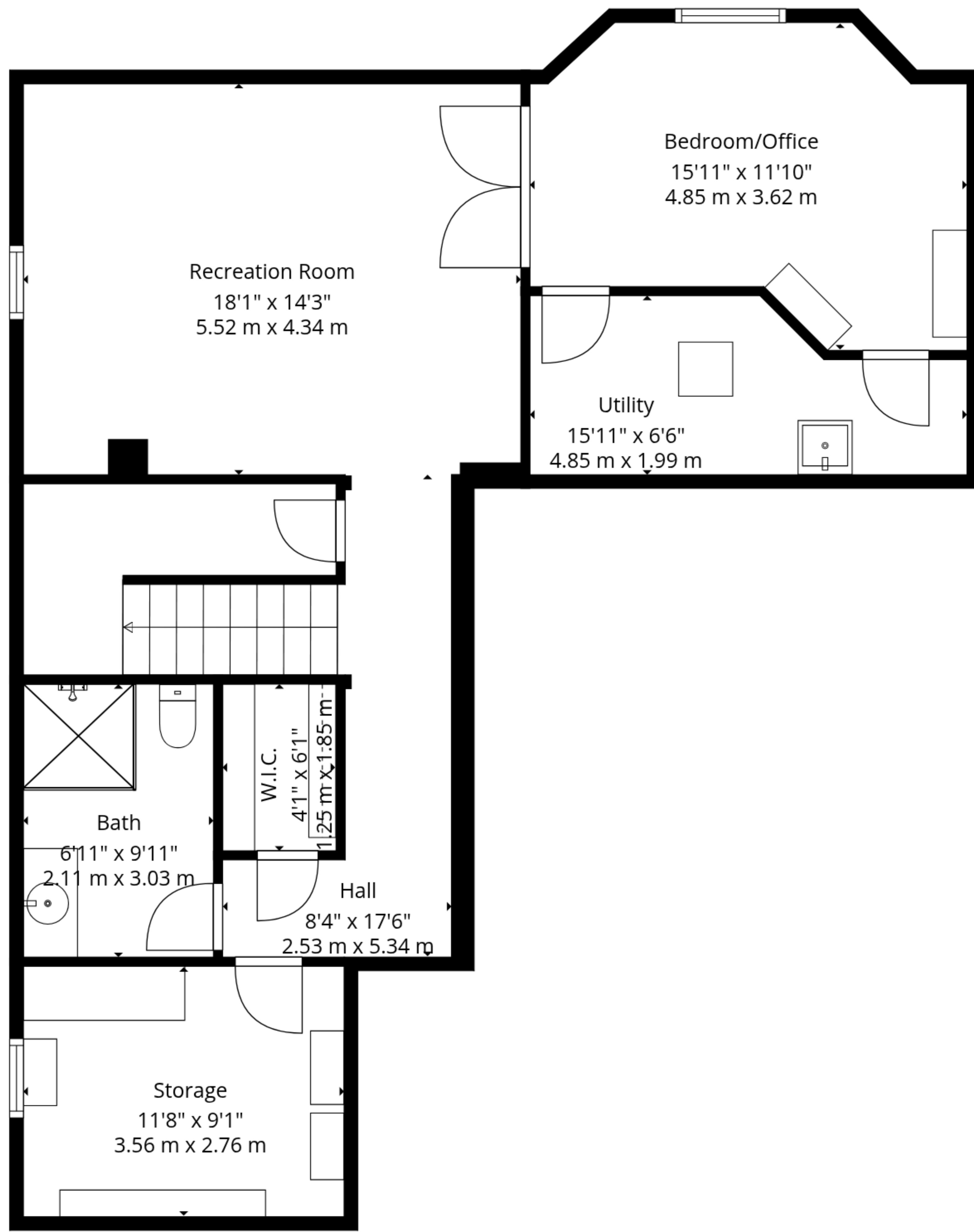
Basement 1
