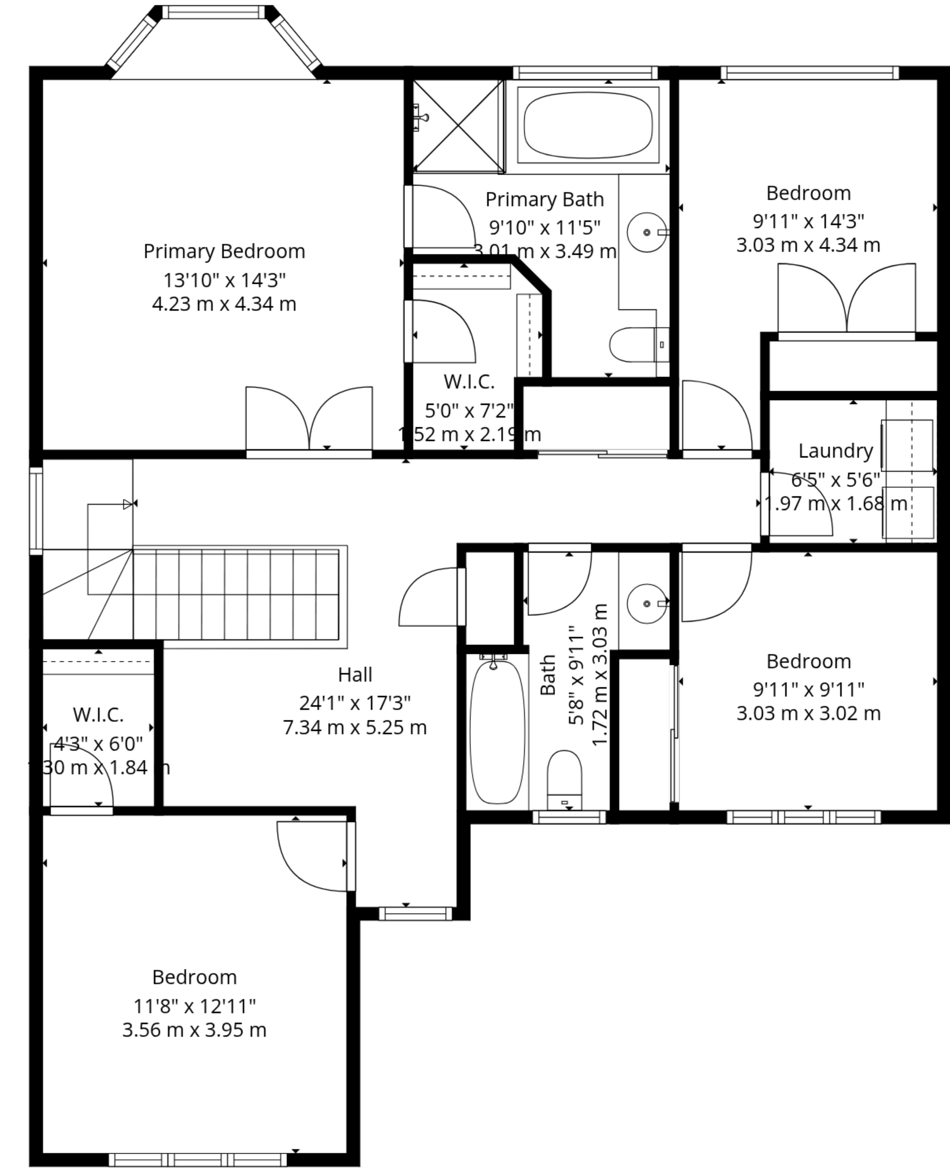
2nd Floor
