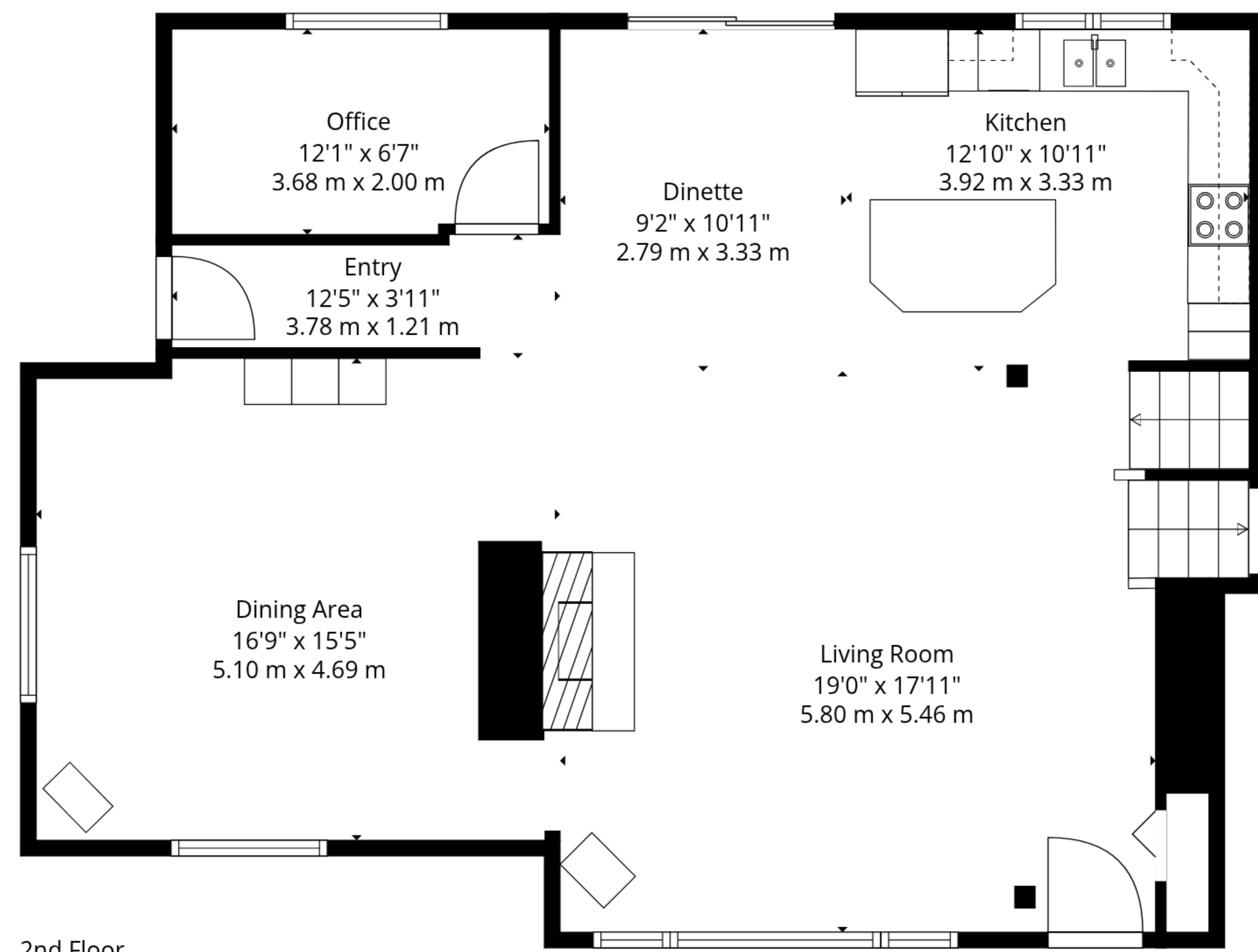
2nd Floor
