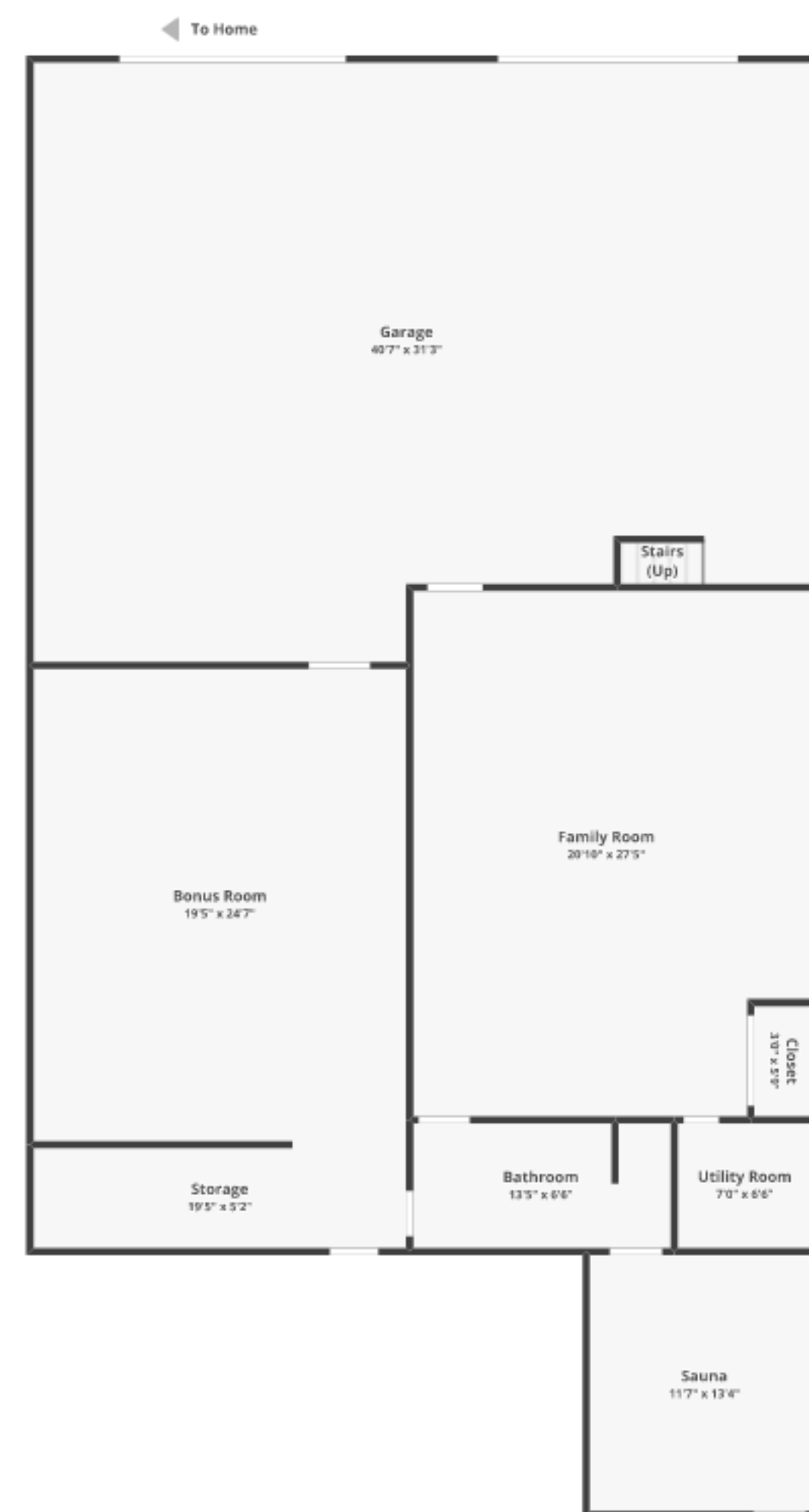
DETACHED GARAGE
